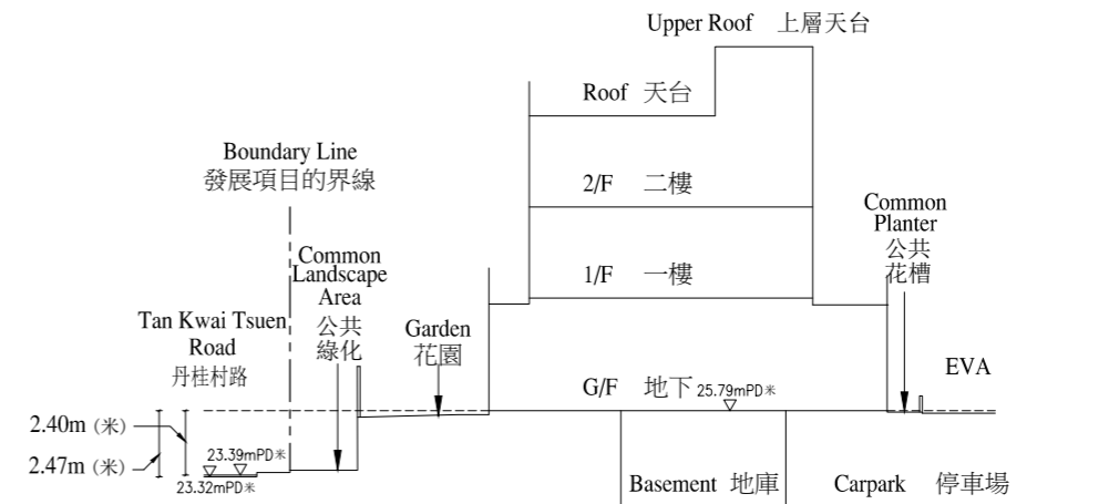
Cross-section Plan (10) 橫截面圖 (10)
