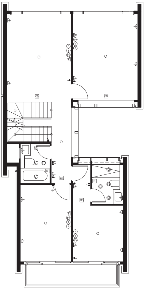
HOUSE 2 — SECOND FLOOR 2號洋房二樓
