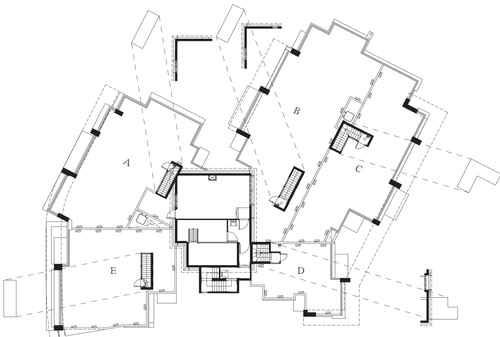
TOWER 16 — UNITS A, B, C, D AND E OF R/F
