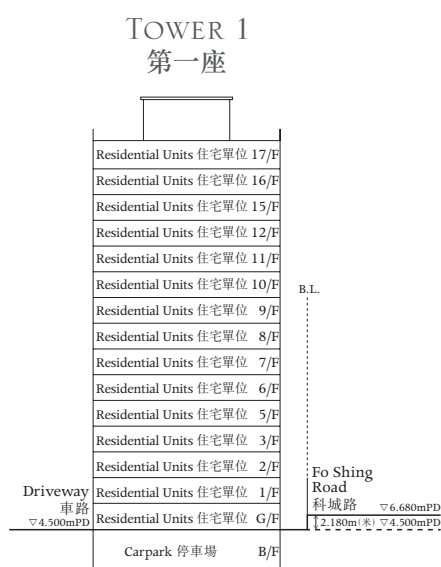
CROSS-SECTION PLAN A1 橫截面圖 A1
