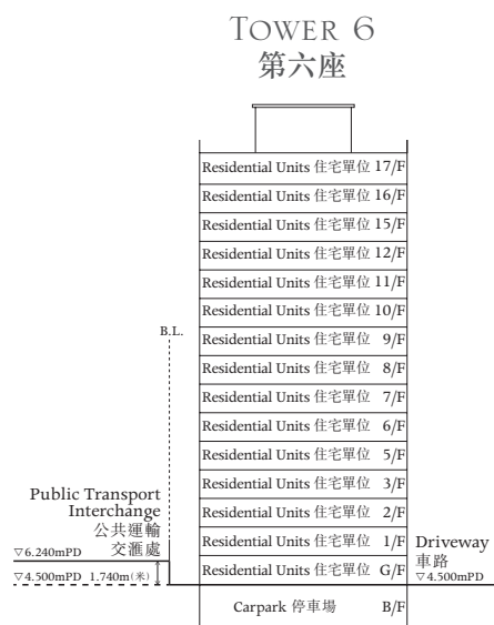
CROSS-SECTION PLAN E 橫截面圖 E
