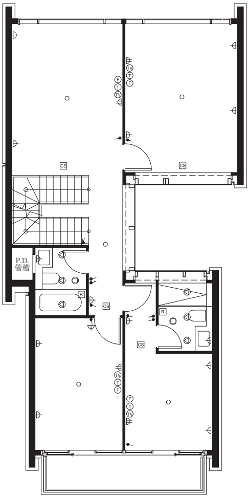
HOUSE 6 — SECOND FLOOR 6號洋房二樓
