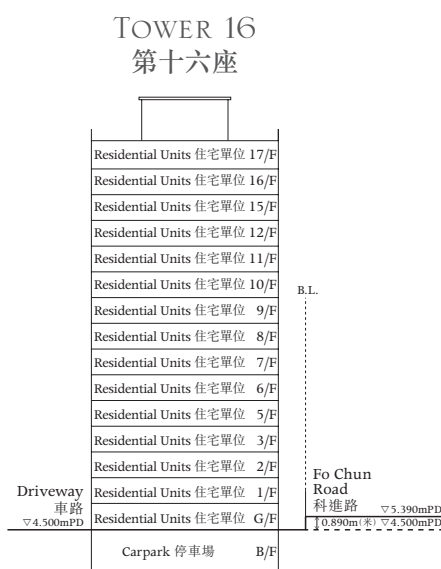
CROSS-SECTION PLAN M2 橫截面圖 M2
