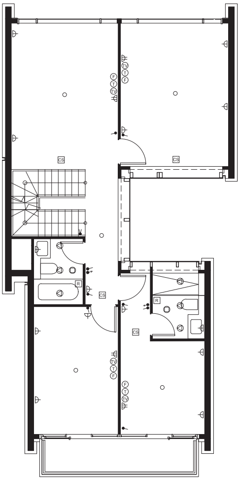
HOUSE 3 — SECOND FLOOR 3號洋房二樓
