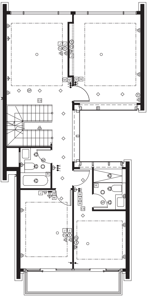
HOUSE 8 — SECOND FLOOR 8號洋房二樓
