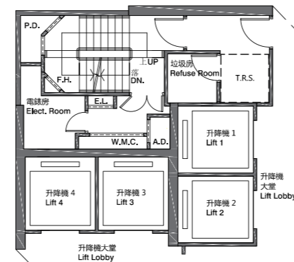
11樓及16樓之部分平面圖 PART PLAN FOR 11/F AND 16/F ONLY
