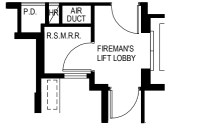
PART PLAN FOR 20/F TO 21/F 20樓至21樓部分平面圖
