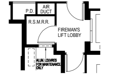
PART PLAN FOR 3/F TO 7/F 3樓至7樓部分平面圖
