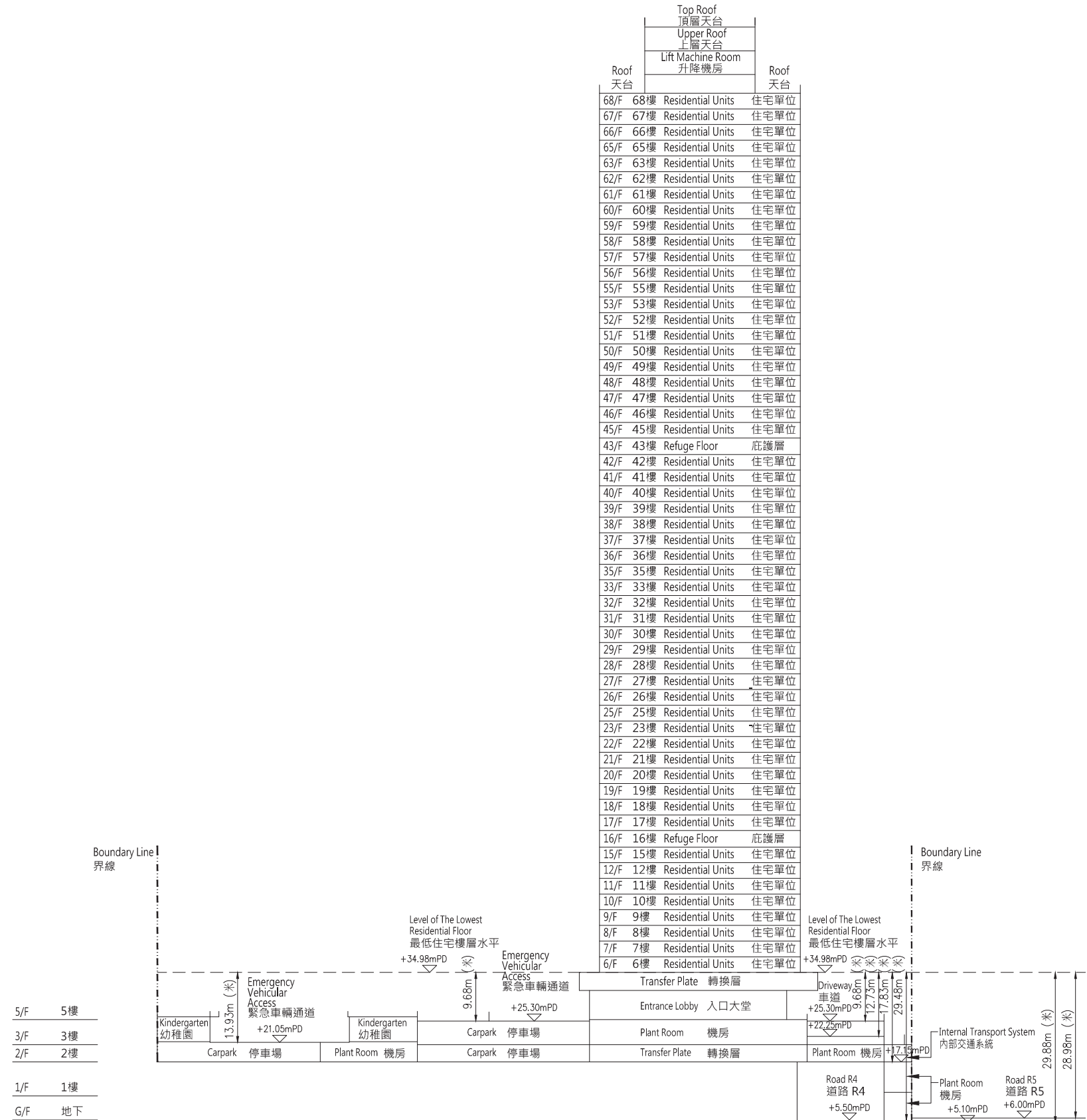
Cross-Section Plan T3 橫截面圖T3
