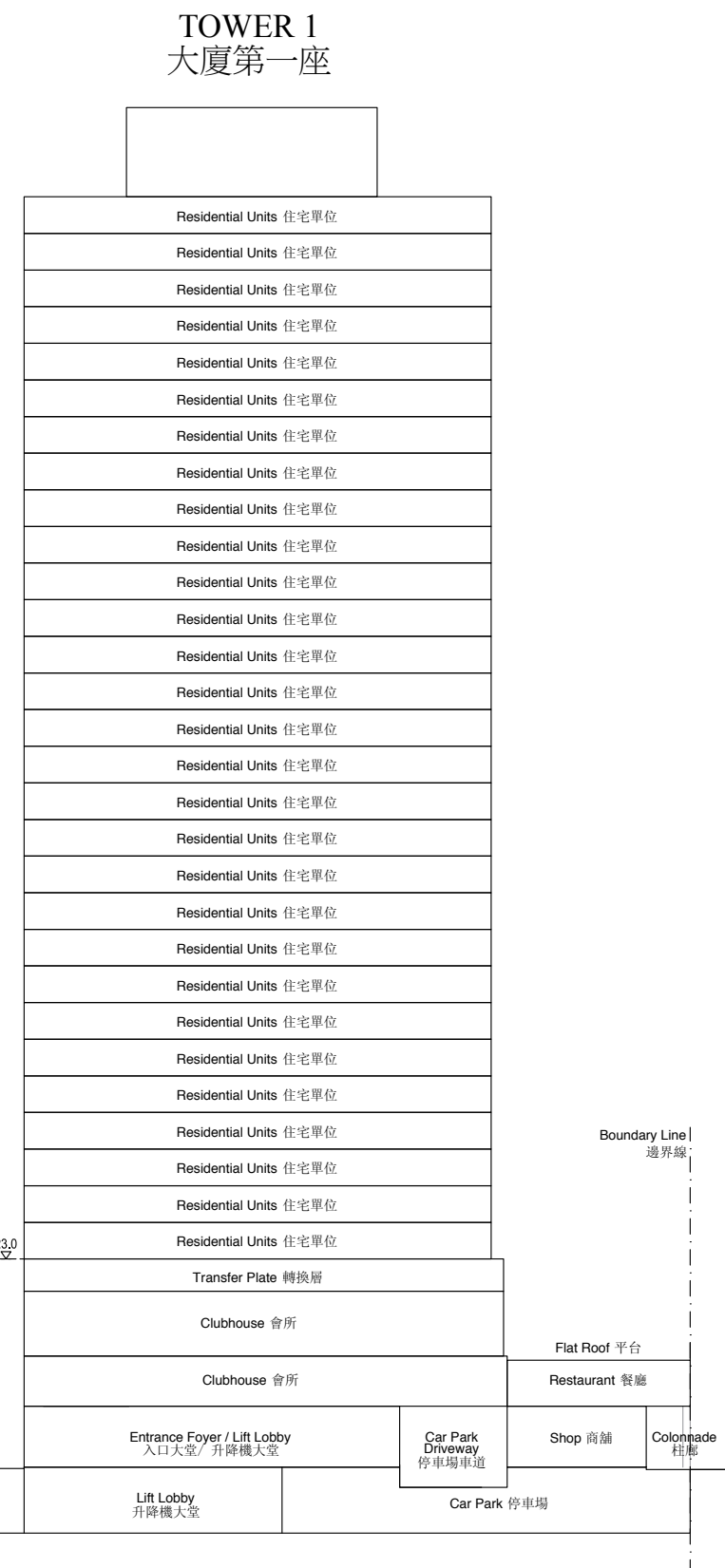
CROSS - SECTION A - A 橫截面圖 A - A
